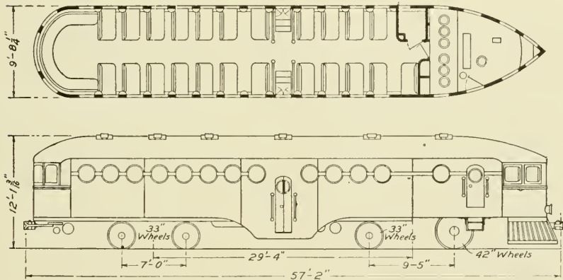
Fig. 9. Plan and Elevation of McKen Motor Passenger Car.
